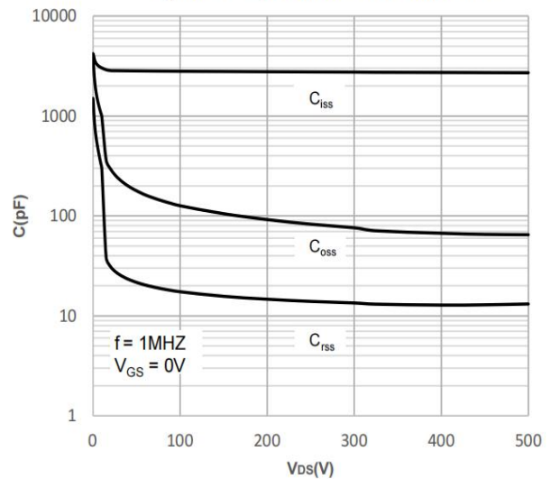
Figure 6: Capacitance Characteristics
