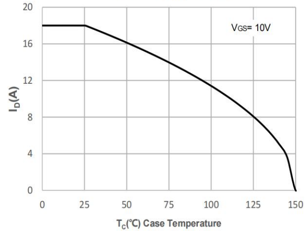
Figure 10: Maximum Continuous Drianc Current vs. Case Temperature
